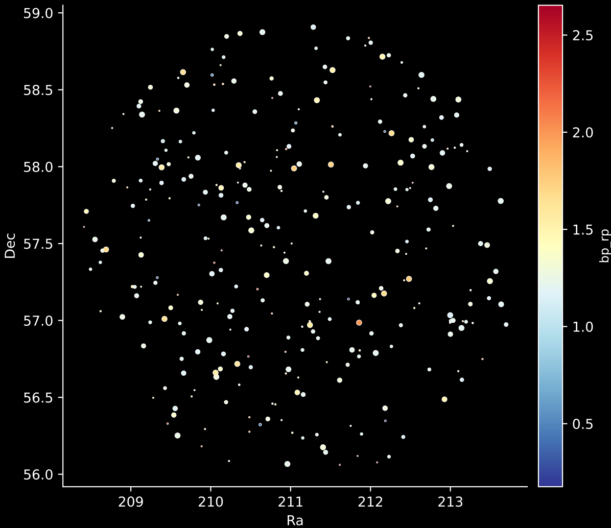
APOGEE DR17 Field: [159+26_btx] Stars: 299
