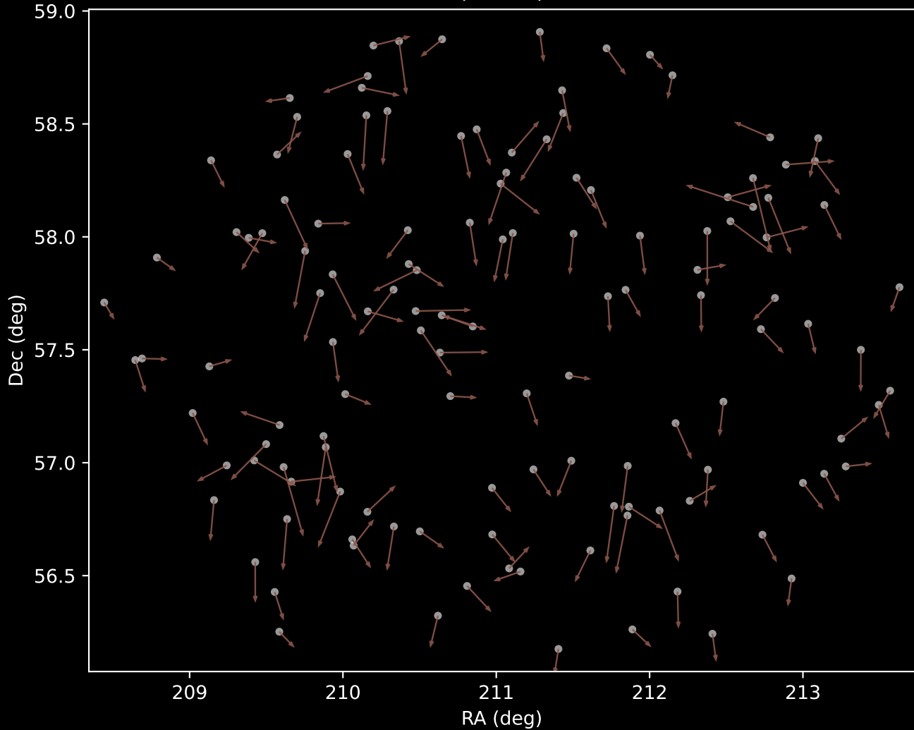
APOGEE DR17 Cluster 10 Proper Motion Vectors (n=130)
