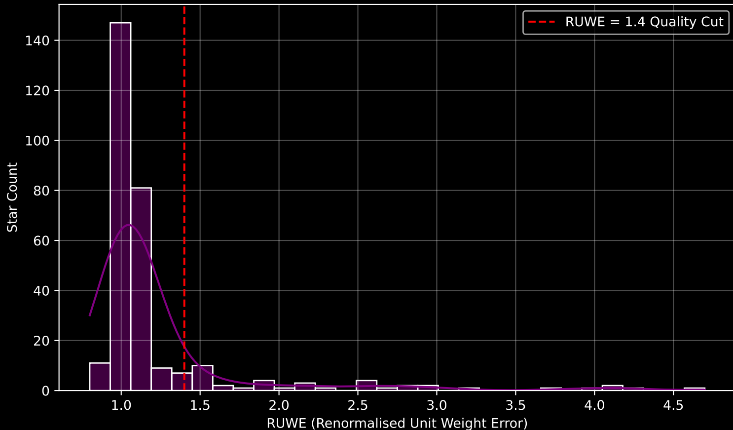
GAPOGEE DR17 Field [159+26_btx] RUWE Distribution (n= 293)
