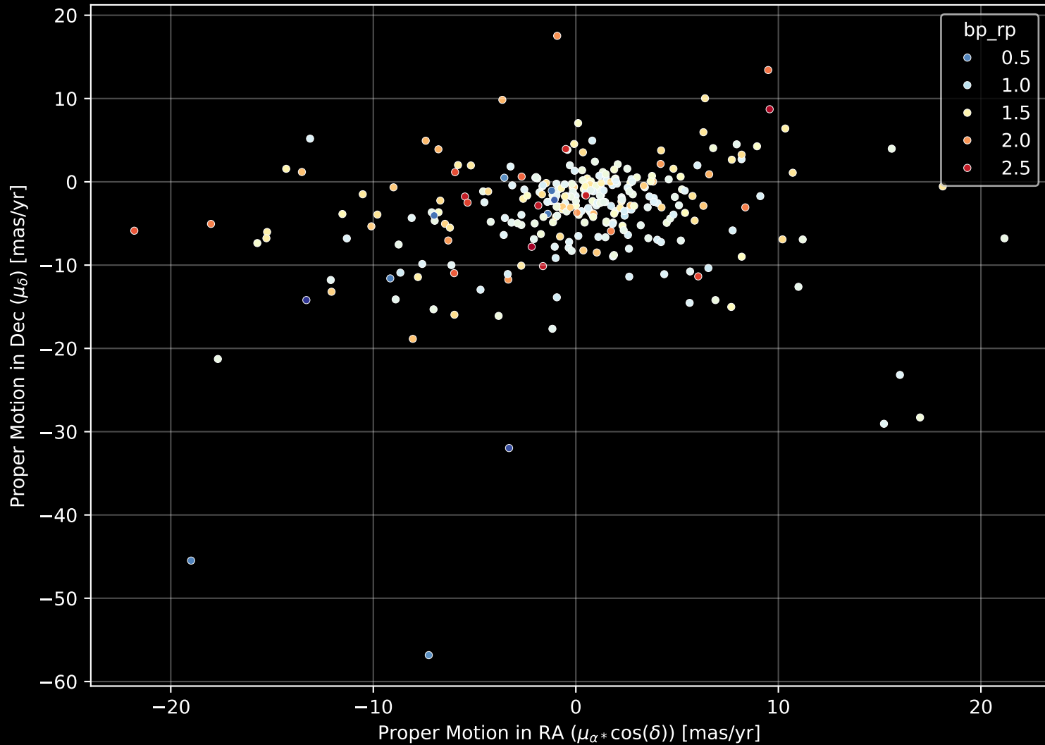
APOGEE DR17 Field: [159+26_btx] Proper Motion Diagram (n= 299)
