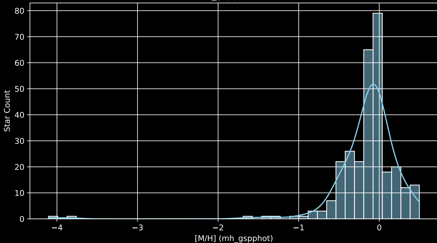
APOGEE DR17 Field: [159+26_btx [M/H] (mh_gspphot) (n= 297)
