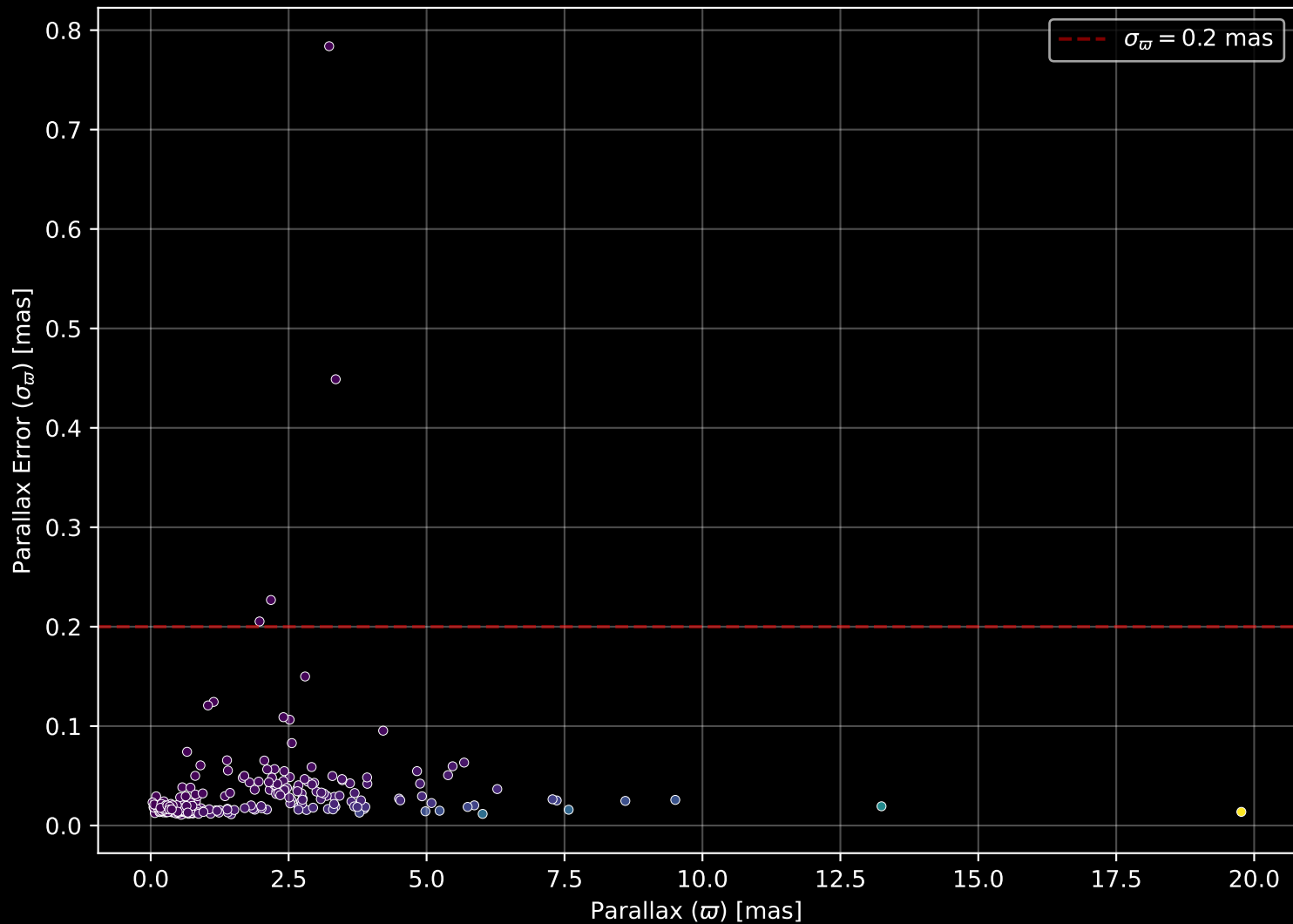
APOGEE DR17 Field: [159+26_btx] Parallax Quality (n= 299)
