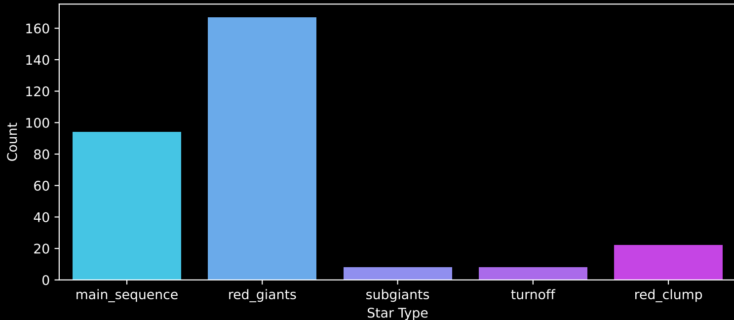
APOGEE DR17 Field: [159+26_btx] Count plot of Star Type
