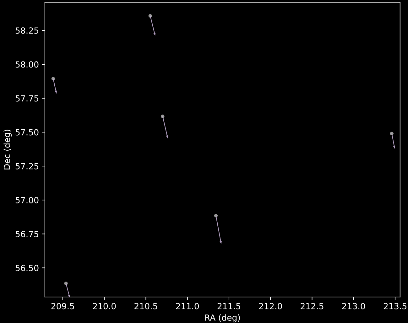
APOGEE DR17 Cluster 9 Proper Motion Vectors (n=6)
